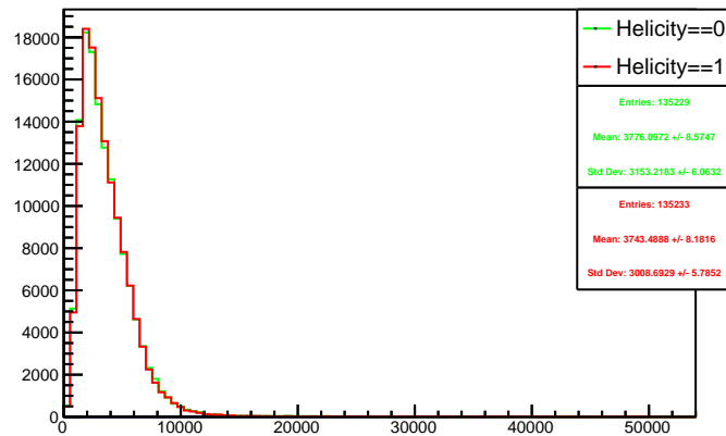
Run 4451 triggerwise, sums: Beam ON, Laser OFF
