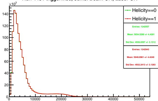
Run 4451 triggerwise, sums: Beam ON, Laser ON
