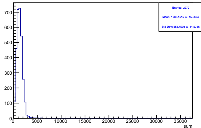
Run 4451 triggerwise, sums: Beam ON, Laser OFF
