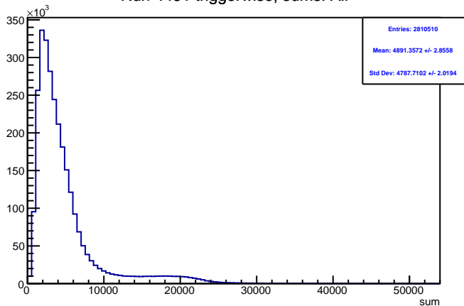
Run 4451 triggerwise, sums: All
