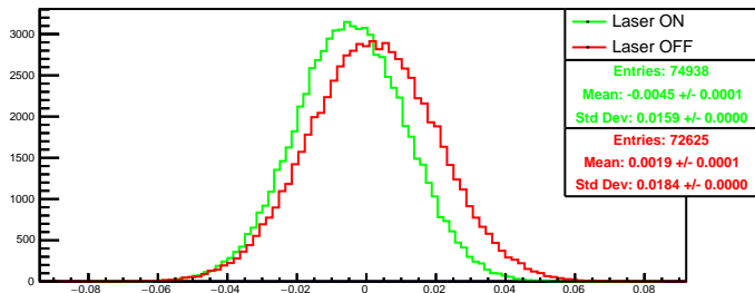
Run 4454 quartetwise, asym4: Beam ON
