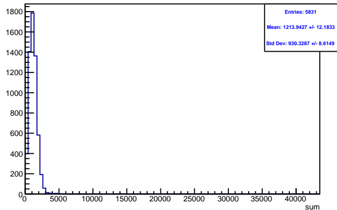
Run 4454 triggerwise, sums: Beam ON, Laser OFF
