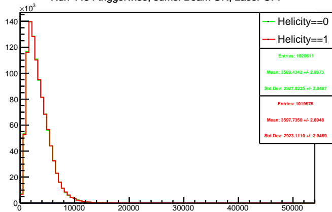
Run 4454 triggerwise, sums: Beam ON, Laser OFF
