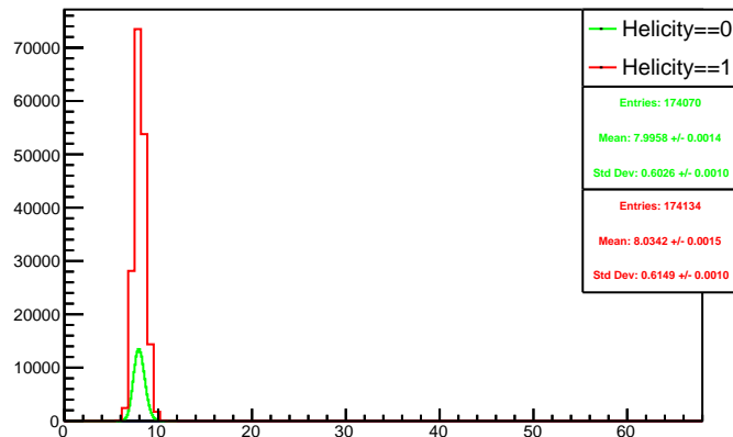
Run 4455 mpwise, acc0: Beam ON, Laser OFF
