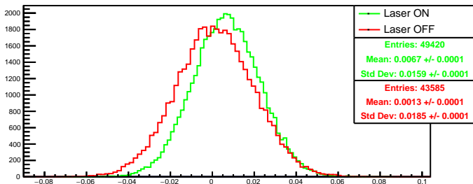
Run 4456 quartetwise, asym4: Beam ON
