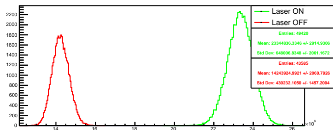
Run 4456 quartetwise, negH4: Beam ON
