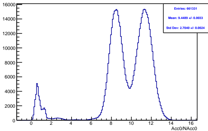
Run 4459 mpwise, acc0: All
