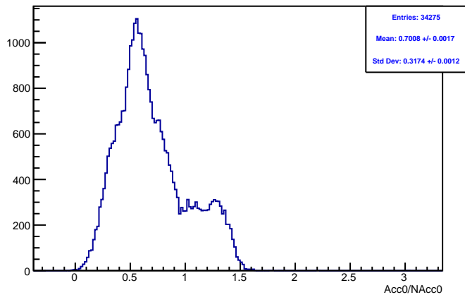
Run 4459 mpwise, acc0: Beam ON, Laser OFF
