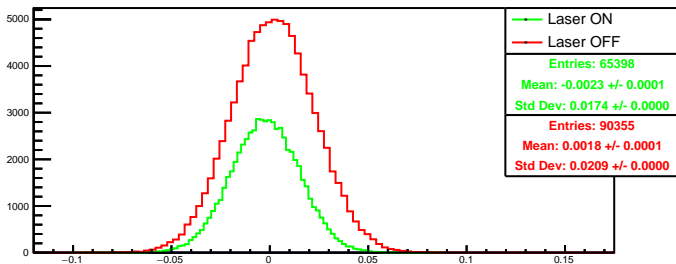
Run 4461 quartetwise, asym0: Beam ON
