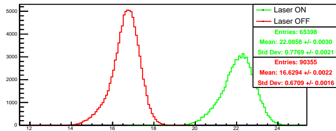
Run 4461 quartetwise, summ0: Beam ON
