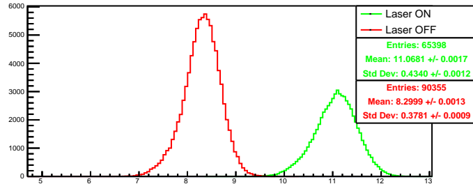
Run 4461 quartetwise, negH0: Beam ON
