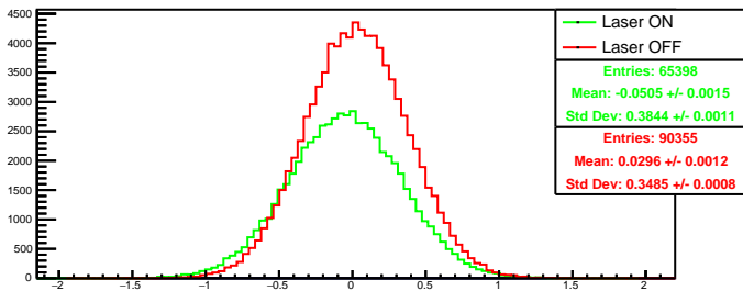
Run 4461 quartetwise, diff0: Beam ON
