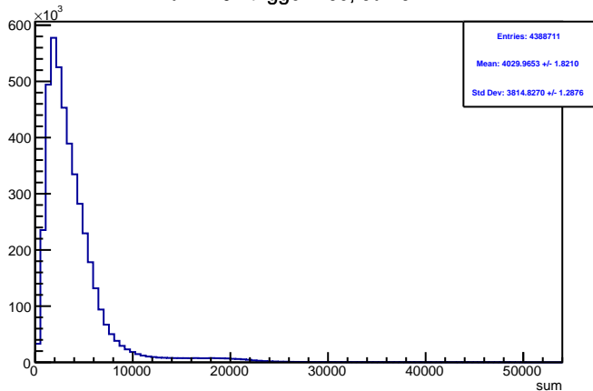
Run 4461 triggerwise, sums: All
