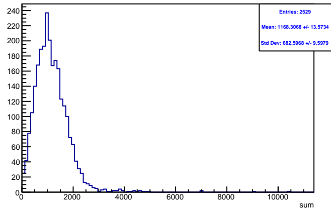
Run 4461 triggerwise, sums: Beam ON, Laser OFF
