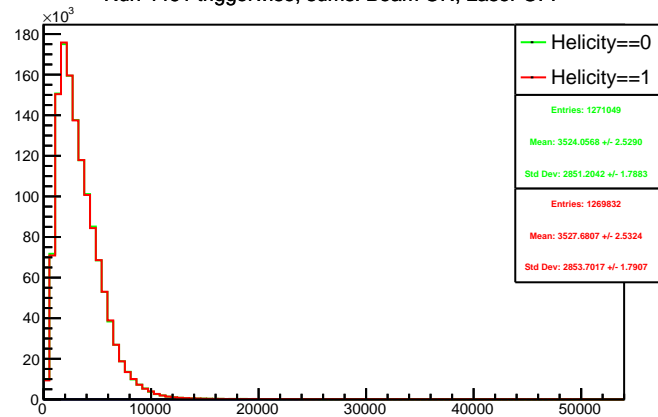
Run 4461 triggerwise, sums: Beam ON, Laser OFF
