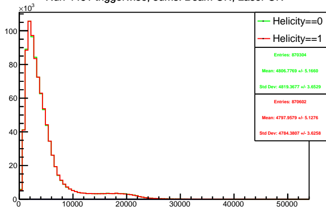
Run 4461 triggerwise, sums: Beam ON, Laser ON
