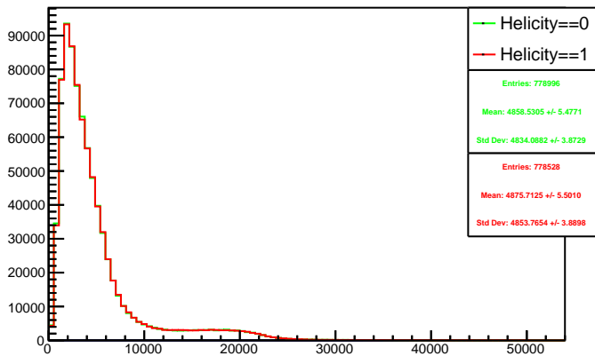
Run 4462 triggerwise, sums: Beam ON, Laser ON
