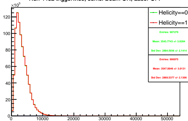
Run 4462 triggerwise, sums: Beam ON, Laser OFF
