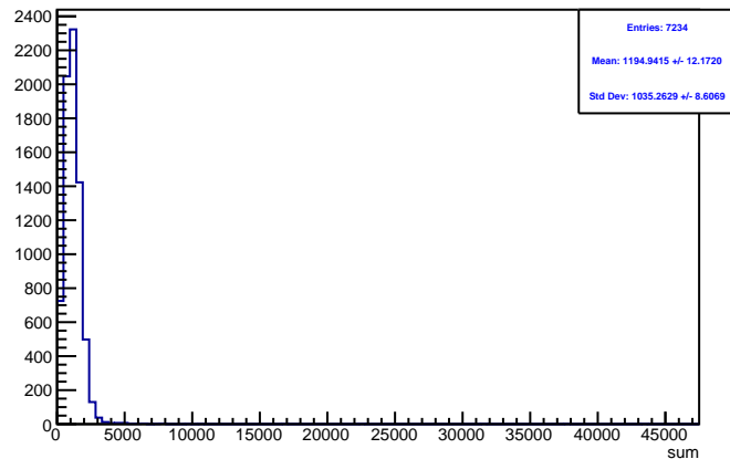
Run 4462 triggerwise, sums: Beam OFF
