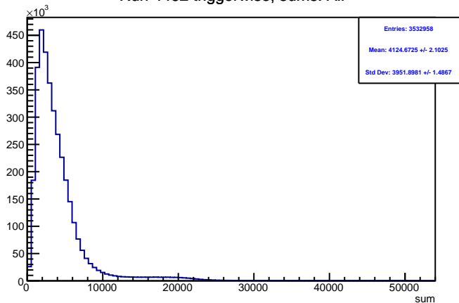
Run 4462 triggerwise, sums: All
