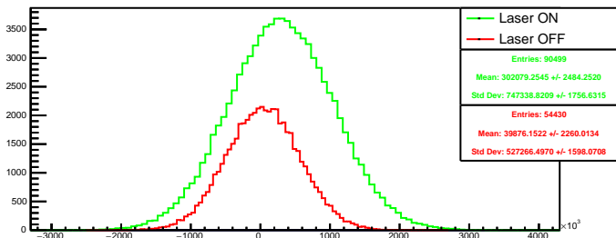
Run 4465 quartetwise, diff4: Beam ON
