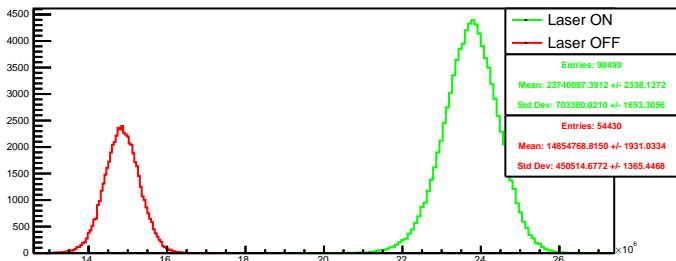
Run 4465 quartetwise, posH4: Beam ON
