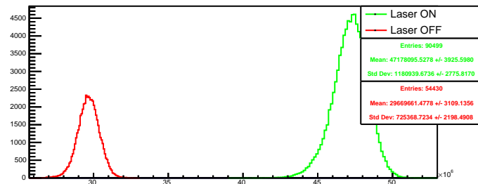
Run 4465 quartetwise, summ4: Beam ON
