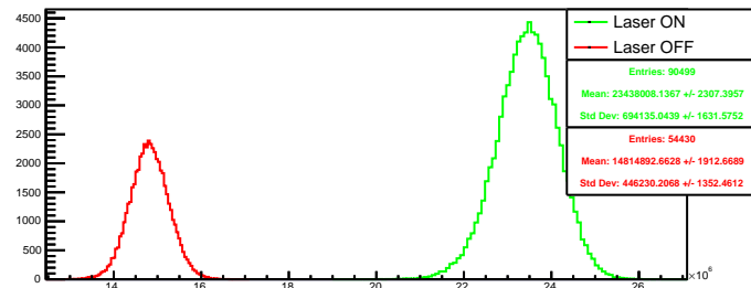
Run 4465 quartetwise, negH4: Beam ON
