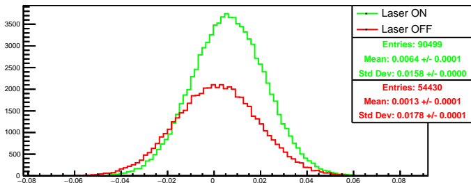
Run 4465 quartetwise, asym4: Beam ON
