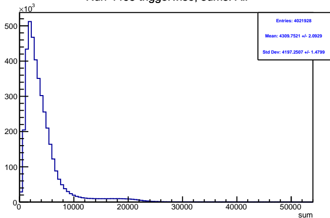
Run 4465 triggerwise, sums: All
