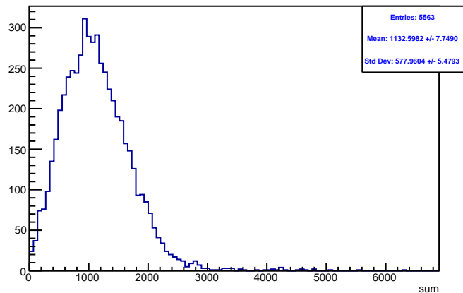
Run 4465 triggerwise, sums: Beam ON, Laser OFF
