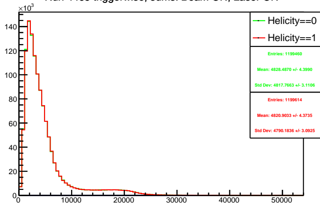
Run 4465 triggerwise, sums: Beam ON, Laser ON
