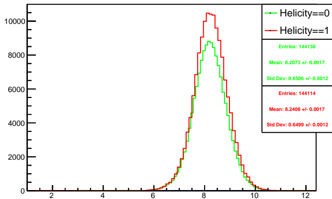
Run 4467 mpwise, acc0: Beam ON, Laser OFF
