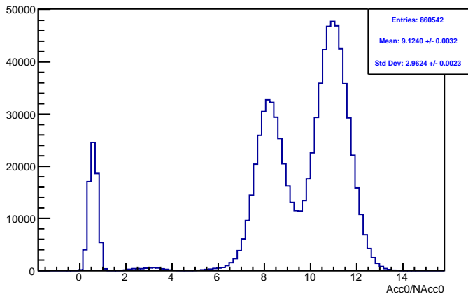
Run 4467 mpwise, acc0: All
