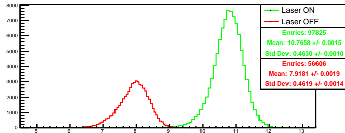
Run 4468 quartetwise, negH0: Beam ON
