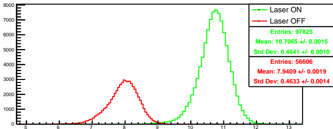
Run 4468 quartetwise, posH0: Beam ON
