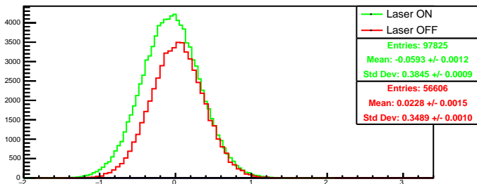
Run 4468 quartetwise, diff0: Beam ON
