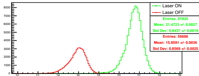
Run 4468 quartetwise, summ0: Beam ON
