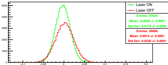
Run 4468 quartetwise, asym0: Beam ON
