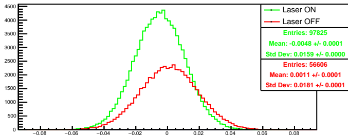
Run 4468 quartetwise, asym4: Beam ON
