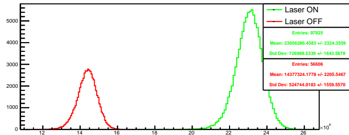
Run 4468 quartetwise, negH4: Beam ON
