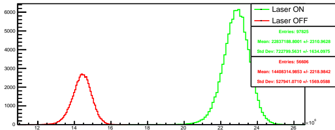
Run 4468 quartetwise, posH4: Beam ON
