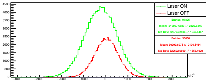
Run 4468 quartetwise, diff4: Beam ON
