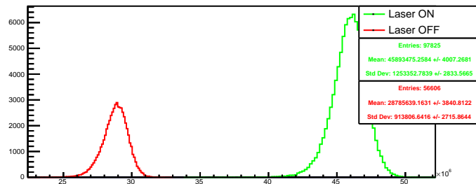
Run 4468 quartetwise, summ4: Beam ON
