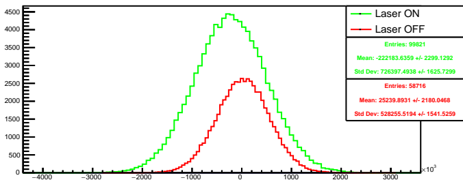
Run 4469 quartetwise, diff4: Beam ON
