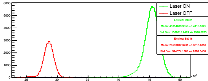
Run 4469 quartetwise, summ4: Beam ON
