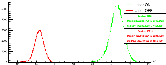
Run 4469 quartetwise, posH4: Beam ON
