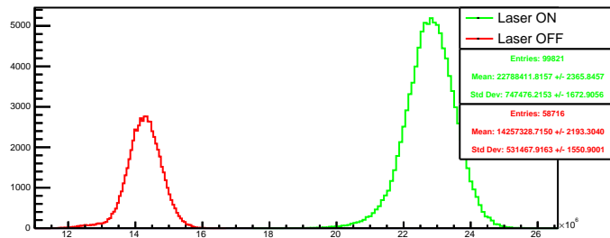
Run 4469 quartetwise, negH4: Beam ON
