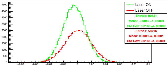
Run 4469 quartetwise, asym4: Beam ON
