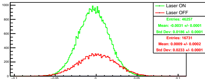
Run 4471 quartetwise, asym0: Beam ON
