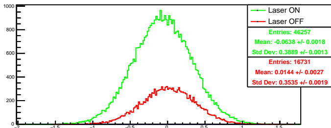
Run 4471 quartetwise, diff0: Beam ON
