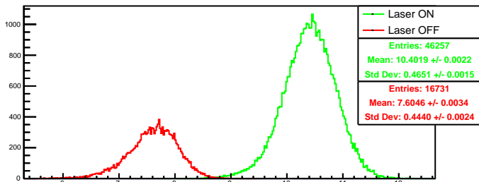
Run 4471 quartetwise, posH0: Beam ON
