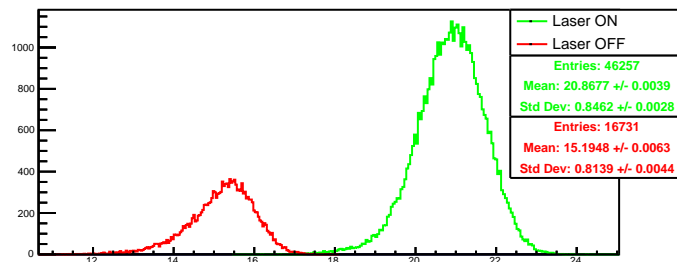
Run 4471 quartetwise, summ0: Beam ON
