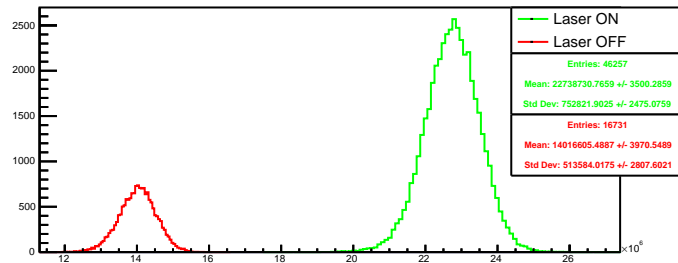
Run 4471 quartetwise, negH4: Beam ON
