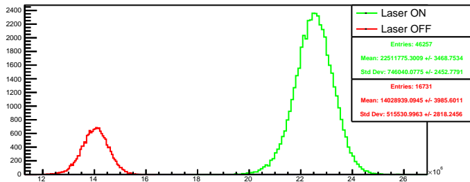
Run 4471 quartetwise, posH4: Beam ON
