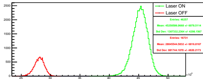
Run 4471 quartetwise, summ4: Beam ON
