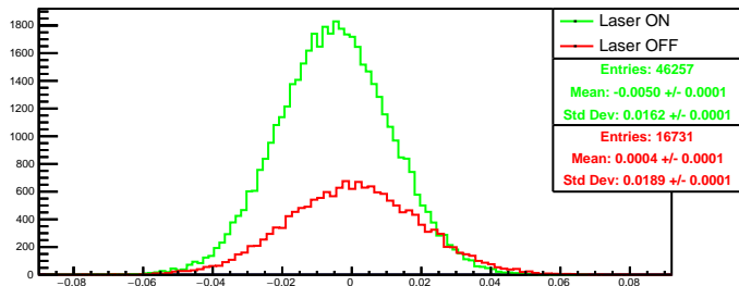
Run 4471 quartetwise, asym4: Beam ON
