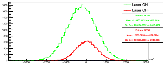
Run 4471 quartetwise, diff4: Beam ON
