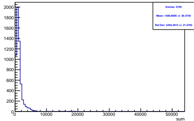
Run 4471 triggerwise, sums: Beam ON, Laser OFF
