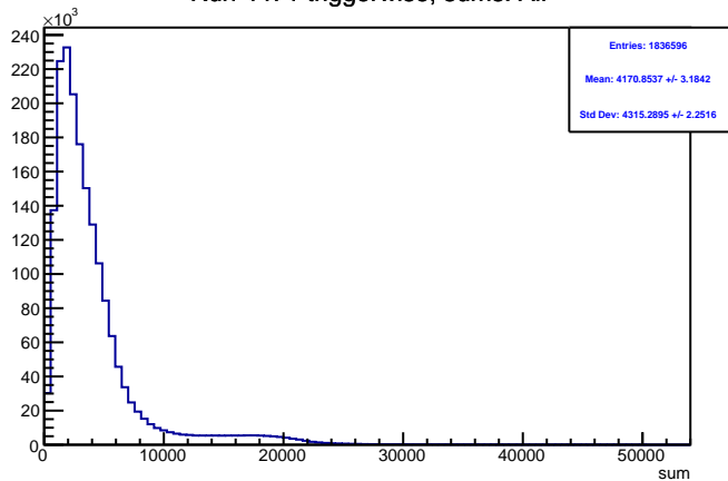
Run 4471 triggerwise, sums: All
