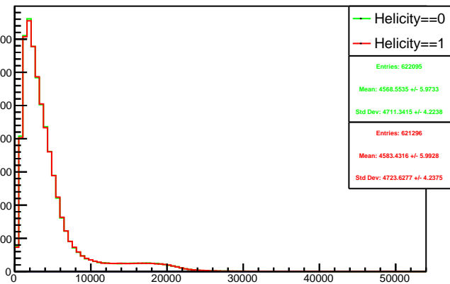
Run 4471 triggerwise, sums: Beam ON, Laser ON
