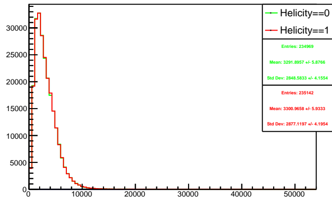
Run 4471 triggerwise, sums: Beam ON, Laser OFF
