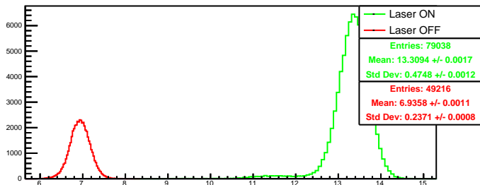
Run 4485 quartetwise, posH0: Beam ON
