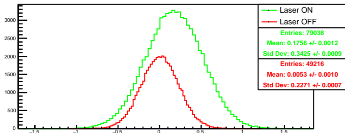
Run 4485 quartetwise, diff0: Beam ON
