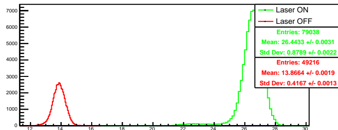
Run 4485 quartetwise, summ0: Beam ON
