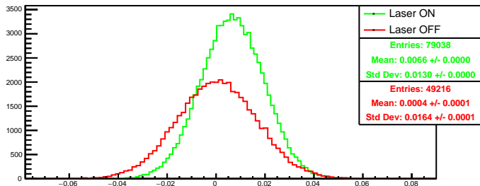
Run 4485 quartetwise, asym0: Beam ON
