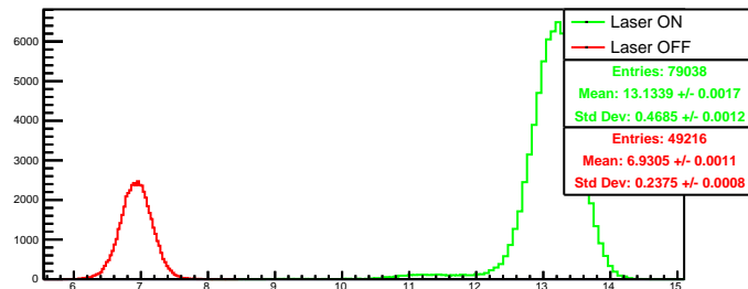
Run 4485 quartetwise, negH0: Beam ON
