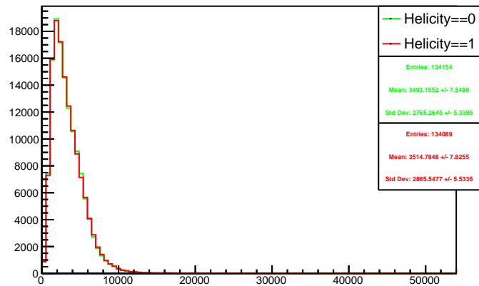
Run 4487 triggerwise, sums: Beam ON, Laser OFF
