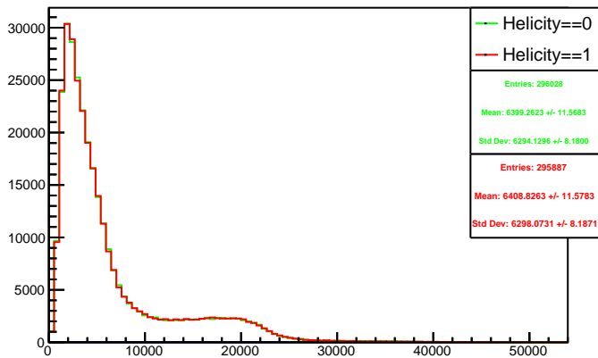
Run 4487 triggerwise, sums: Beam ON, Laser ON
