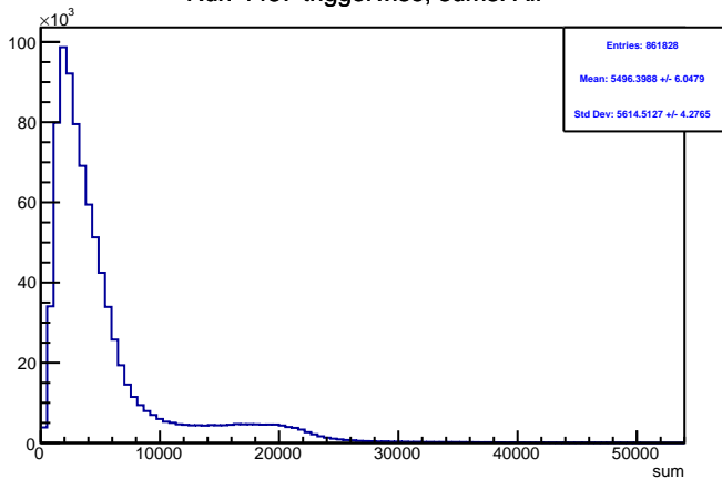
Run 4487 triggerwise, sums: All
