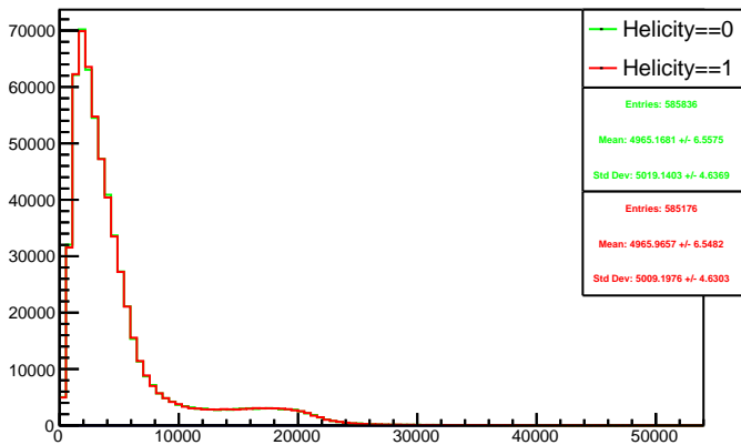
Run 4501 triggerwise, sums: Beam ON, Laser ON
