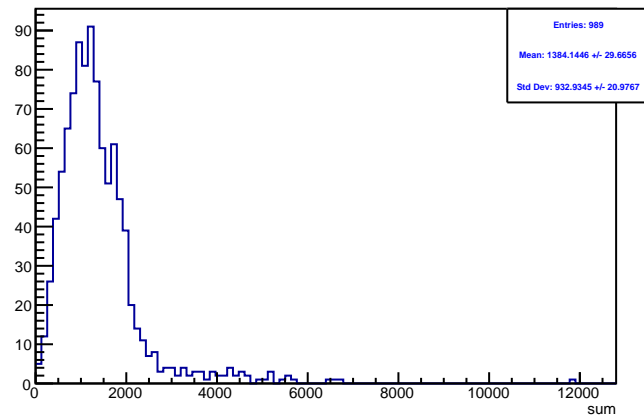
Run 4501 triggerwise, sums: Beam ON, Laser OFF
