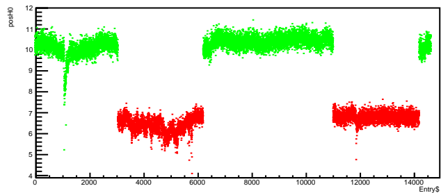
Run 4503 quartetwise, posH0 vs time
