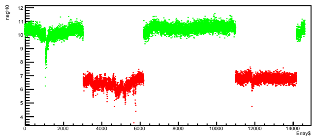
Run 4503 quartetwise, negH0 vs time
