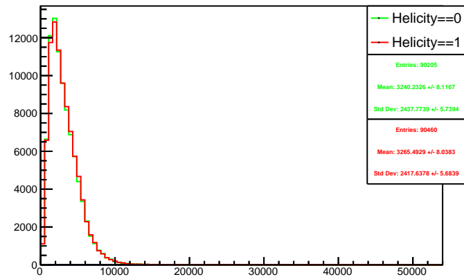
Run 4503 triggerwise, sums: Beam ON, Laser OFF
