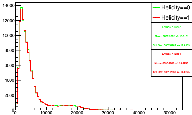
Run 4503 triggerwise, sums: Beam ON, Laser ON
