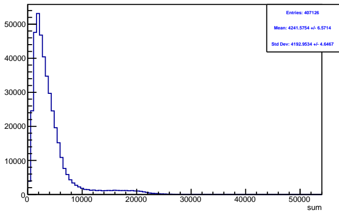
Run 4503 triggerwise, sums: Beam ON, Laser ON
