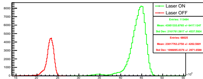
Run 4506 quartetwise, summ4: Beam ON
