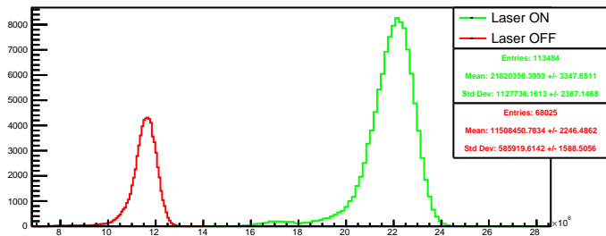
Run 4506 quartetwise, posH4: Beam ON
