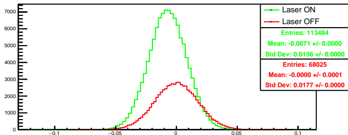
Run 4506 quartetwise, asym4: Beam ON
