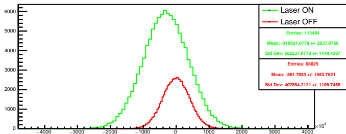
Run 4506 quartetwise, diff4: Beam ON
