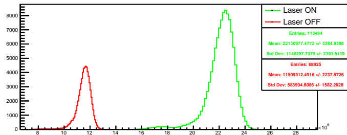
Run 4506 quartetwise, negH4: Beam ON
