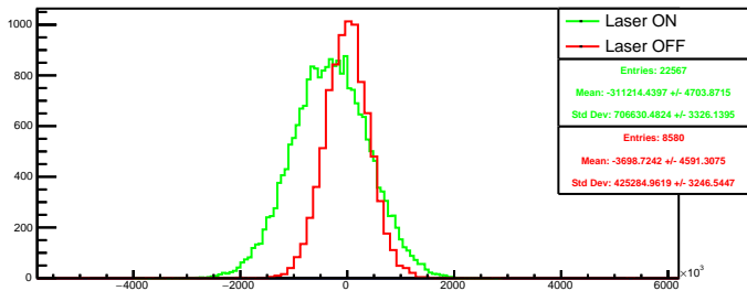
Run 4507 quartetwise, diff4: Beam ON
