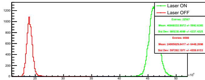
Run 4507 quartetwise, summ4: Beam ON
