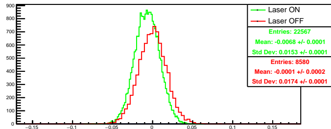
Run 4507 quartetwise, asym4: Beam ON
