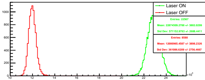
Run 4507 quartetwise, posH4: Beam ON
