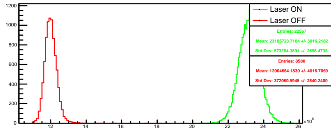
Run 4507 quartetwise, negH4: Beam ON
