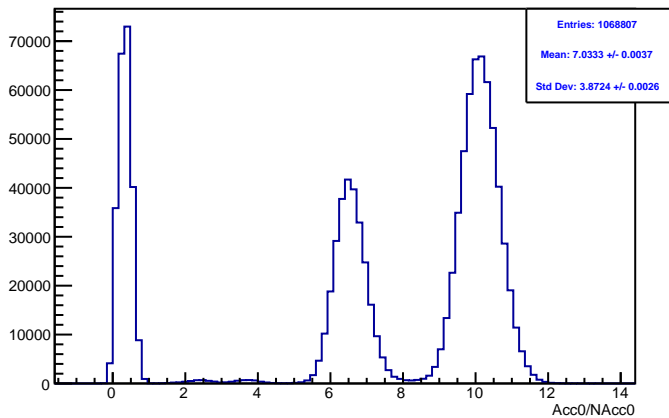
Run 4508 mpwise, acc0: Beam ON, Laser ON
