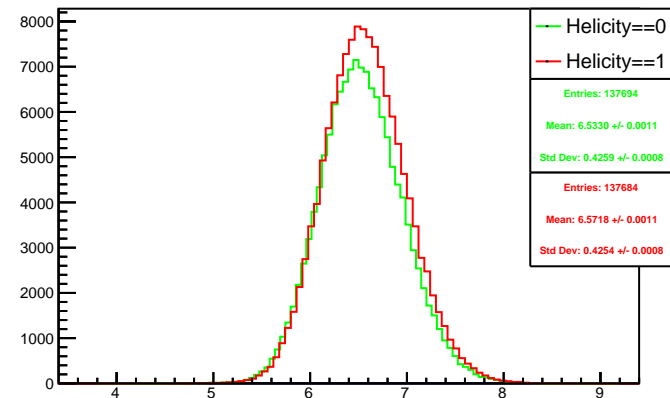
Run 4508 mpwise, acc0: Beam ON, Laser OFF
