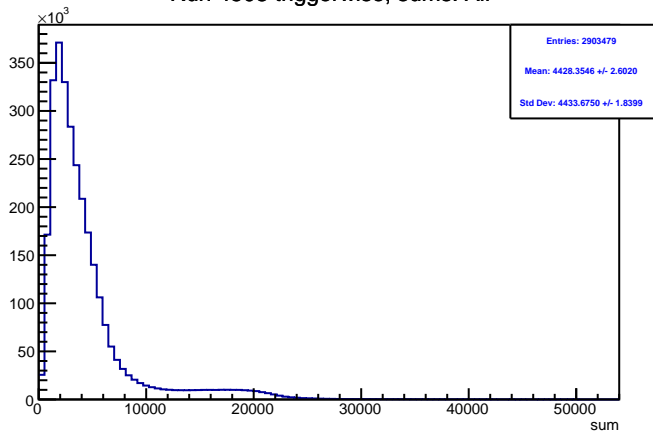
Run 4508 triggerwise, sums: All
