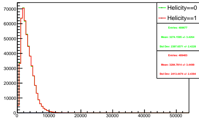
Run 4508 triggerwise, sums: Beam ON, Laser OFF
