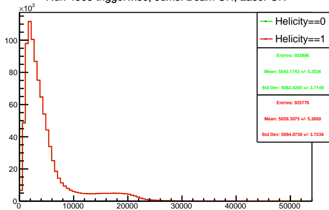
Run 4508 triggerwise, sums: Beam ON, Laser ON
