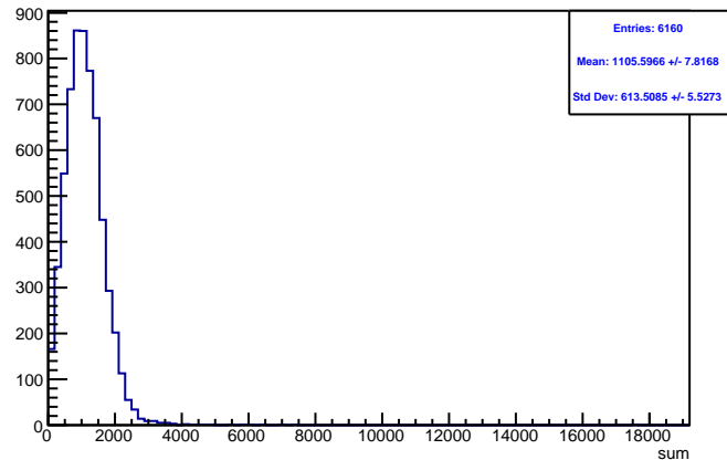
Run 4508 triggerwise, sums: Beam OFF
