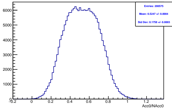
Run 4511 mpwise, acc0: Beam ON, Laser OFF
