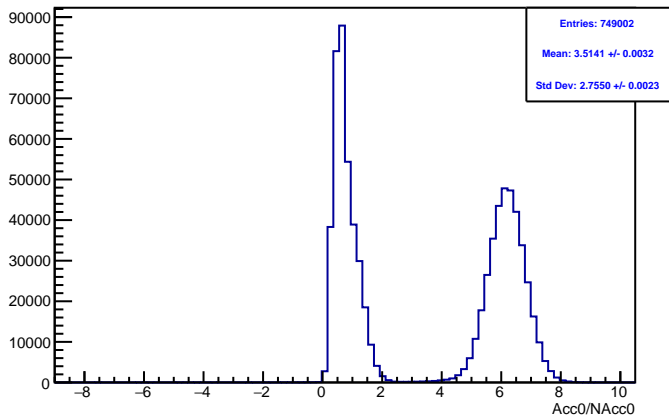
Run 4511 mpwise, acc0: Beam ON, Laser ON
