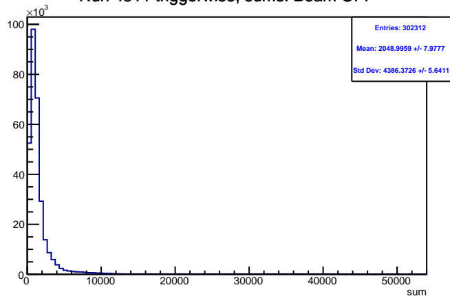
Run 4511 triggerwise, sums: Beam OFF
