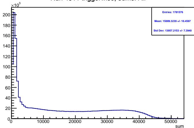
Run 4511 triggerwise, sums: All
