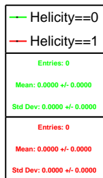
Run 4511 triggerwise, sums: Beam ON, Laser OFF
