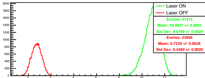
Run 4517 quartetwise, posH0: Beam ON
