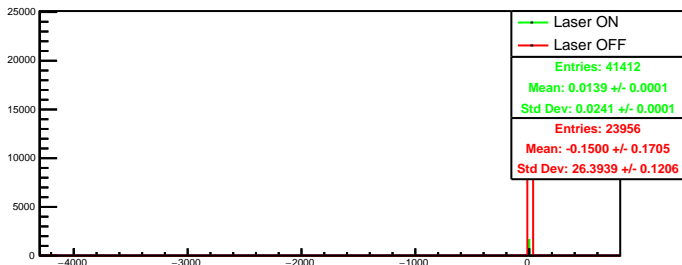
Run 4517 quartetwise, asym0: Beam ON
