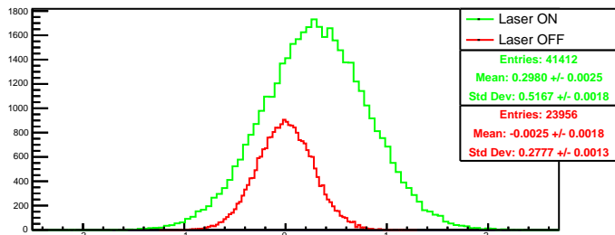
Run 4517 quartetwise, diff0: Beam ON
