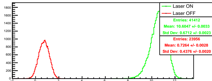
Run 4517 quartetwise, negH0: Beam ON
