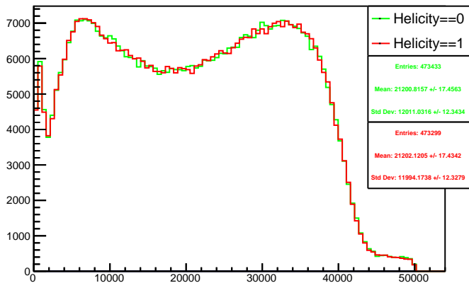
Run 4517 triggerwise, sums: Beam ON, Laser ON
