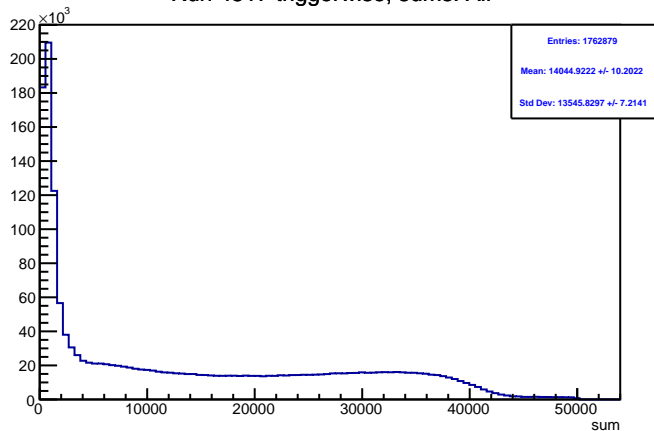
Run 4517 triggerwise, sums: All
