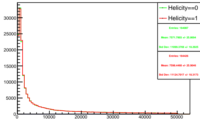
Run 4517 triggerwise, sums: Beam ON, Laser OFF
