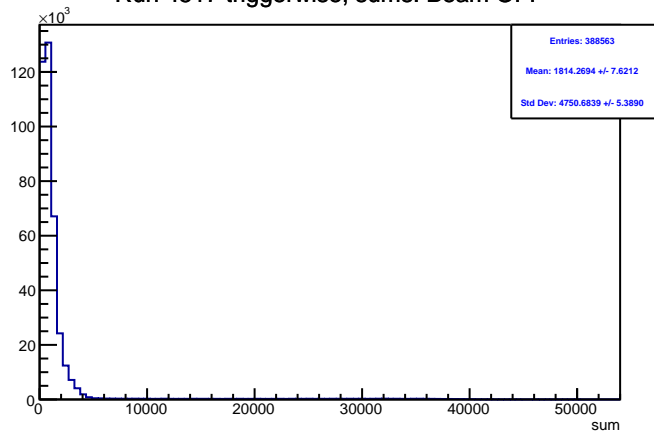
Run 4517 triggerwise, sums: Beam OFF
