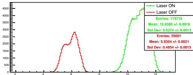
Run 4521 quartetwise, posH0: Beam ON
