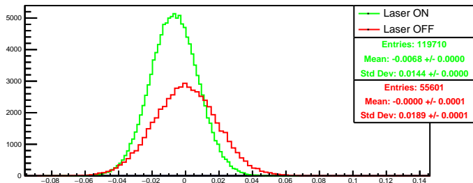
Run 4521 quartetwise, asym0: Beam ON
