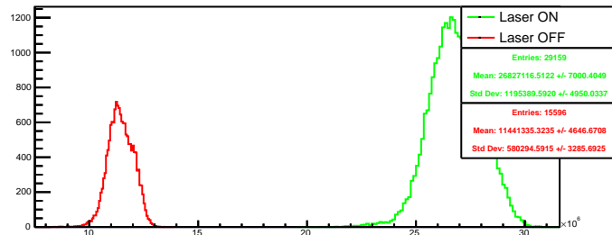
Run 4524 quartetwise, negH4: Beam ON
