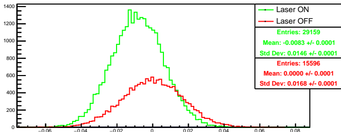
Run 4524 quartetwise, asym4: Beam ON
