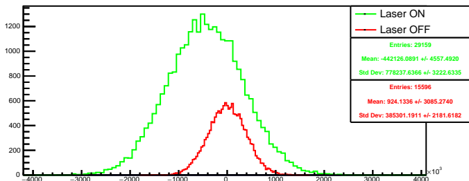
Run 4524 quartetwise, diff4: Beam ON
