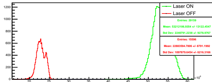
Run 4524 quartetwise, summ4: Beam ON
