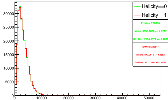
Run 4524 triggerwise, sums: Beam ON, Laser OFF
