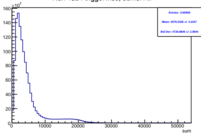
Run 4524 triggerwise, sums: All
