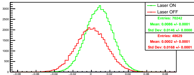
Run 4526 quartetwise, asym4: Beam ON
