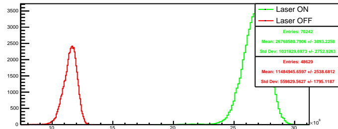
Run 4526 quartetwise, negH4: Beam ON
