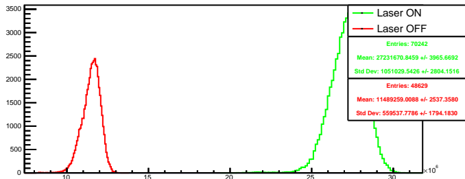
Run 4526 quartetwise, posH4: Beam ON
