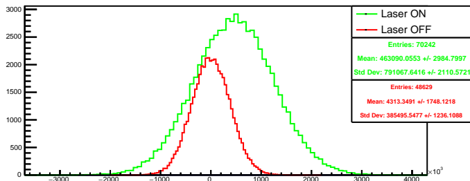
Run 4526 quartetwise, diff4: Beam ON
