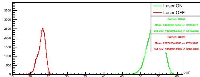
Run 4526 quartetwise, summ4: Beam ON
