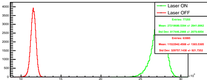
Run 4527 quartetwise, posH4: Beam ON
