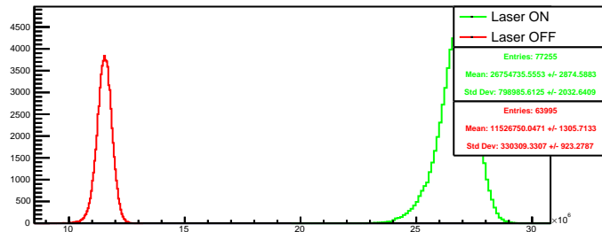
Run 4527 quartetwise, negH4: Beam ON
