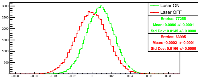
Run 4527 quartetwise, asym4: Beam ON
