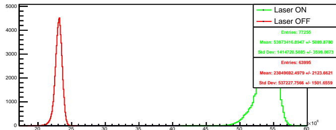
Run 4527 quartetwise, summ4: Beam ON
