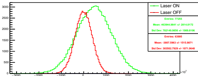
Run 4527 quartetwise, diff4: Beam ON
