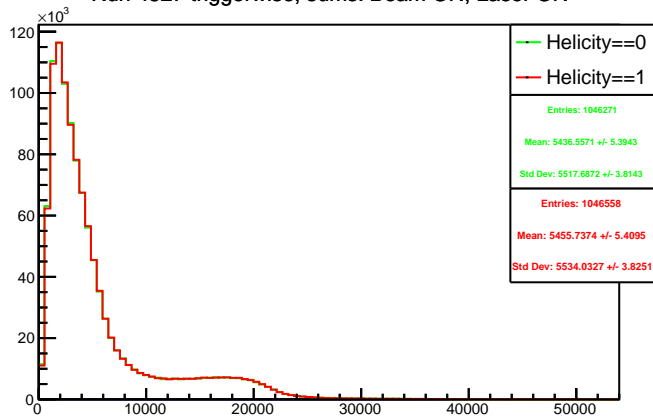
Run 4527 triggerwise, sums: Beam ON, Laser ON
