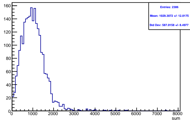
Run 4527 triggerwise, sums: Beam ON, Laser OFF
