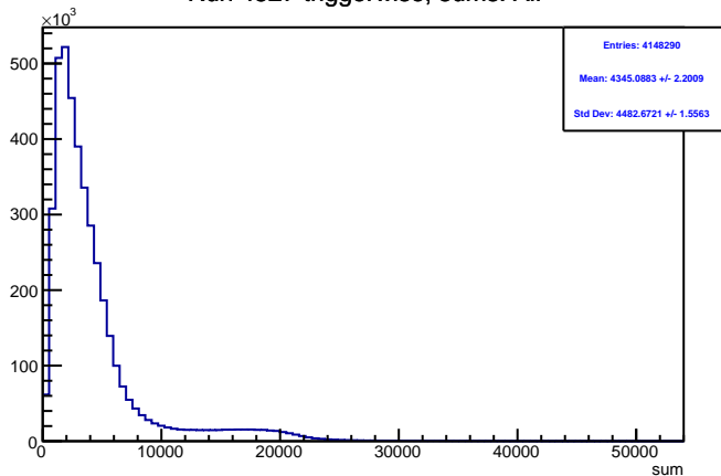
Run 4527 triggerwise, sums: All
