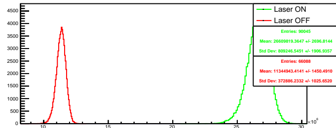
Run 4528 quartetwise, negH4: Beam ON
