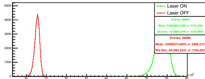
Run 4528 quartetwise, summ4: Beam ON
