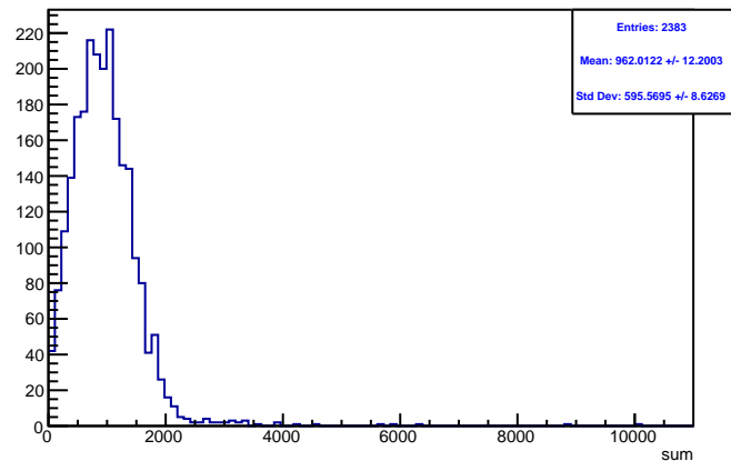
Run 4528 triggerwise, sums: Beam ON, Laser OFF
