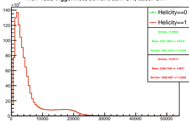
Run 4528 triggerwise, sums: Beam ON, Laser ON
