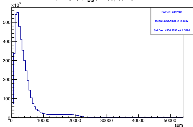
Run 4528 triggerwise, sums: All
