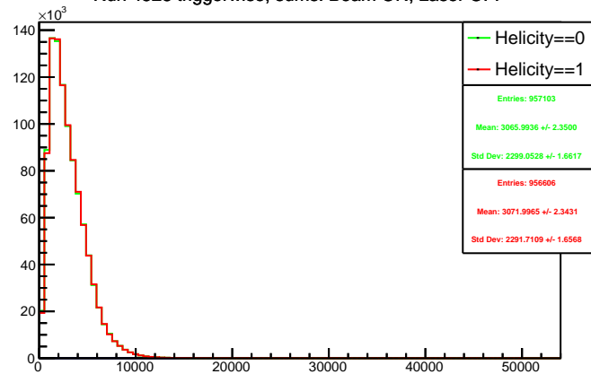
Run 4528 triggerwise, sums: Beam ON, Laser OFF
