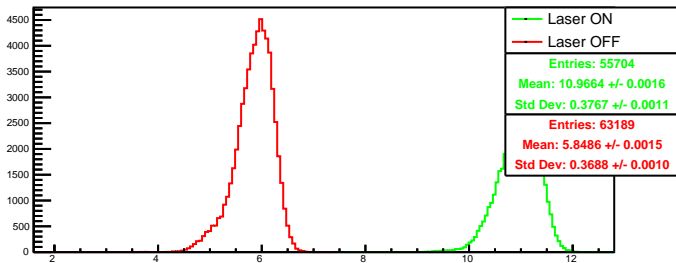
Run 4529 quartetwise, posH0: Beam ON
