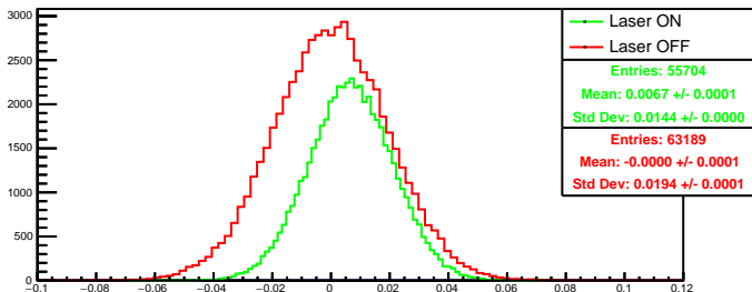
Run 4529 quartetwise, asym0: Beam ON
