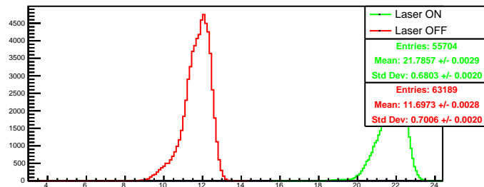
Run 4529 quartetwise, summ0: Beam ON
