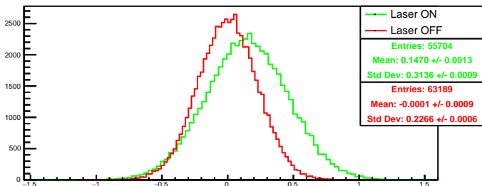
Run 4529 quartetwise, diff0: Beam ON
