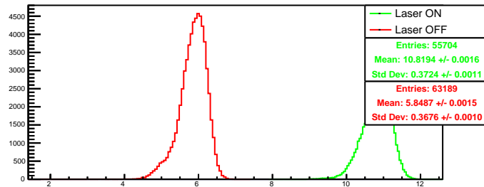
Run 4529 quartetwise, negH0: Beam ON
