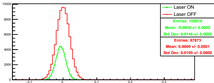
Run 4530 quartetwise, asym0: Beam ON
