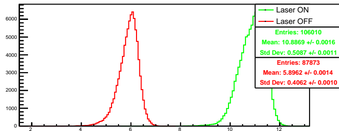
Run 4530 quartetwise, negH0: Beam ON
