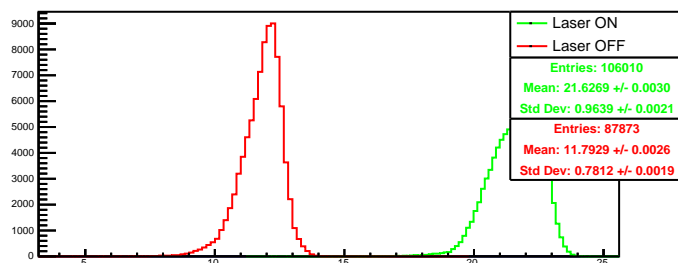
Run 4530 quartetwise, summ0: Beam ON
