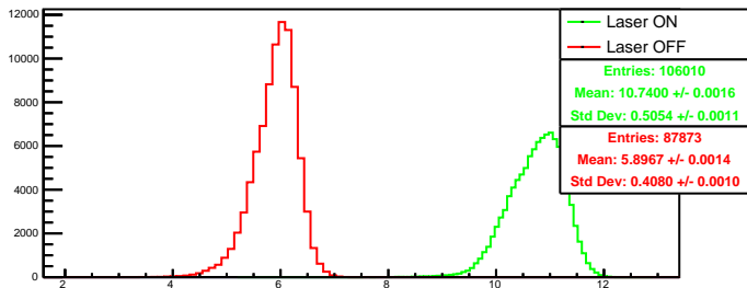
Run 4530 quartetwise, posH0: Beam ON
