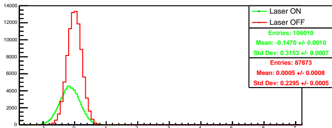
Run 4530 quartetwise, diff0: Beam ON
