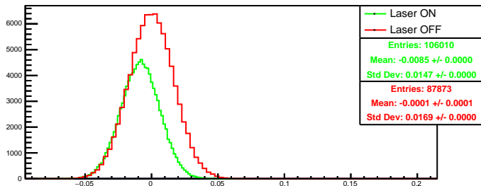
Run 4530 quartetwise, asym4: Beam ON
