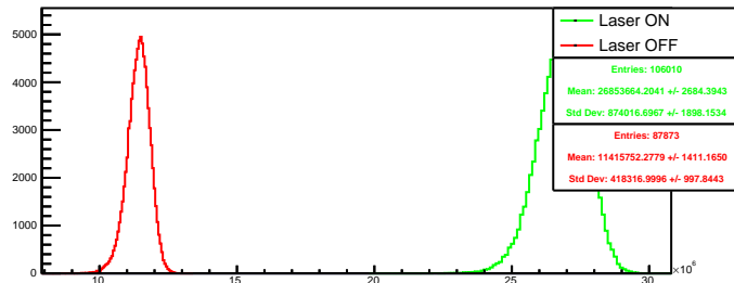
Run 4530 quartetwise, negH4: Beam ON
