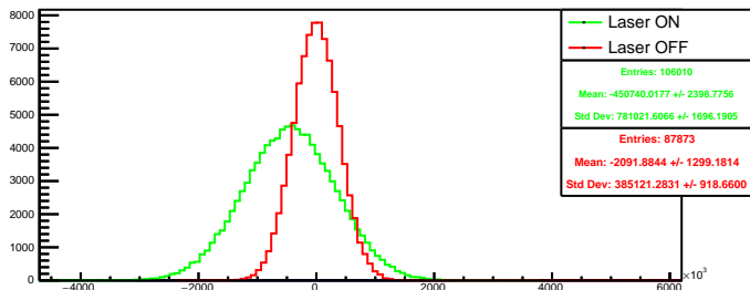
Run 4530 quartetwise, diff4: Beam ON
