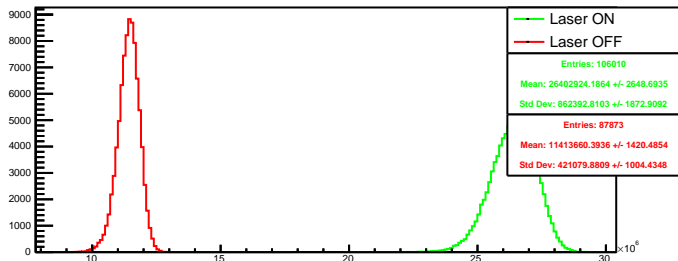
Run 4530 quartetwise, posH4: Beam ON
