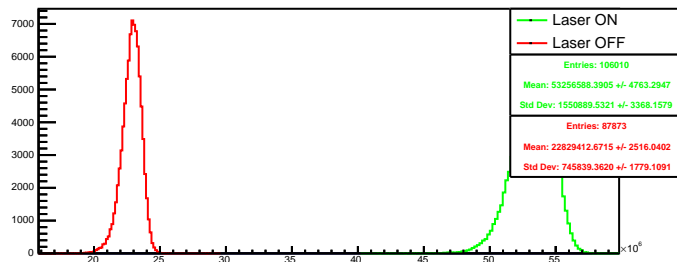
Run 4530 quartetwise, summ4: Beam ON
