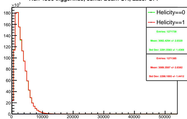
Run 4530 triggerwise, sums: Beam ON, Laser OFF
