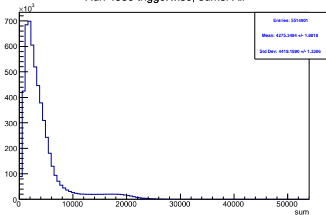
Run 4530 triggerwise, sums: All
