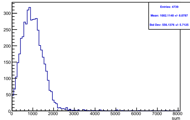
Run 4530 triggerwise, sums: Beam ON, Laser OFF
