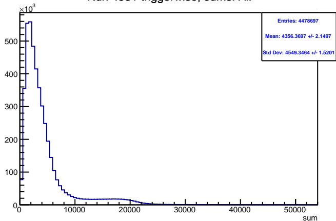
Run 4531 triggerwise, sums: All
