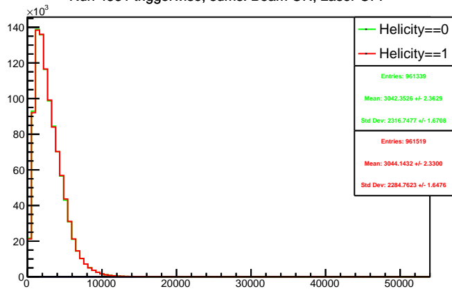
Run 4531 triggerwise, sums: Beam ON, Laser OFF
