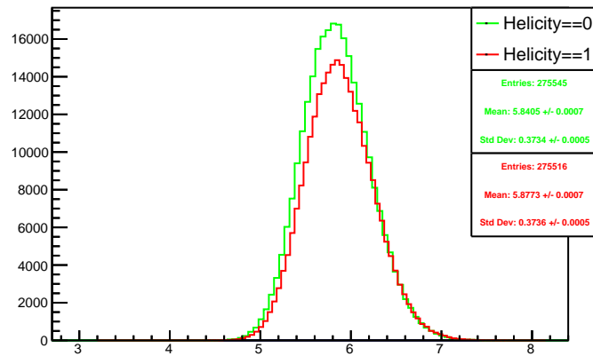
Run 4532 mpwise, acc0: Beam ON, Laser OFF
