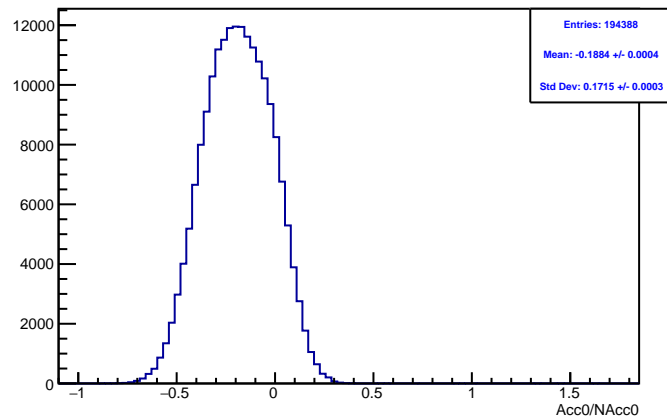
Run 4532 mpwise, acc0: Beam ON, Laser OFF
