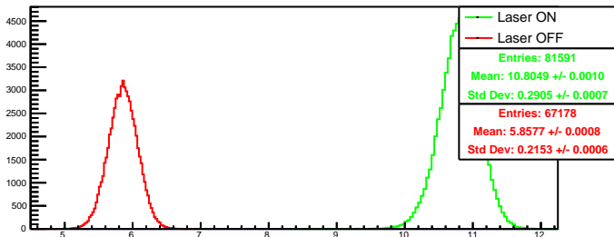
Run 4532 quartetwise, posH0: Beam ON
