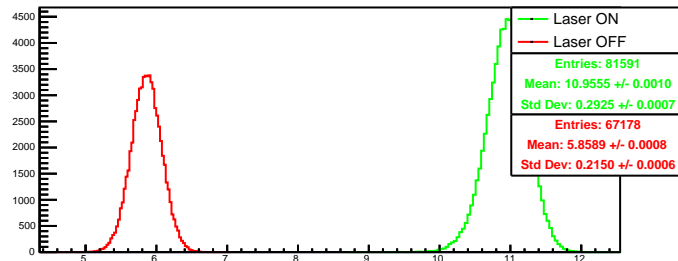
Run 4532 quartetwise, negH0: Beam ON
