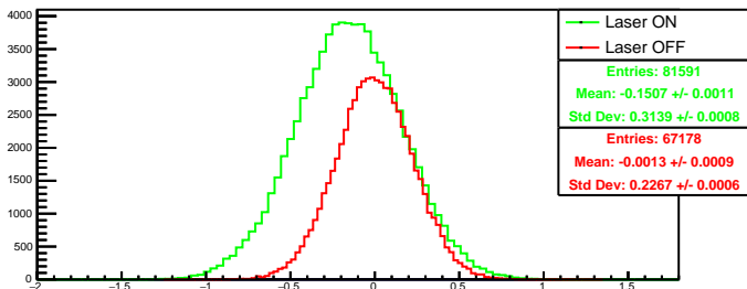
Run 4532 quartetwise, diff0: Beam ON
