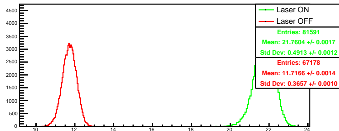
Run 4532 quartetwise, summ0: Beam ON
