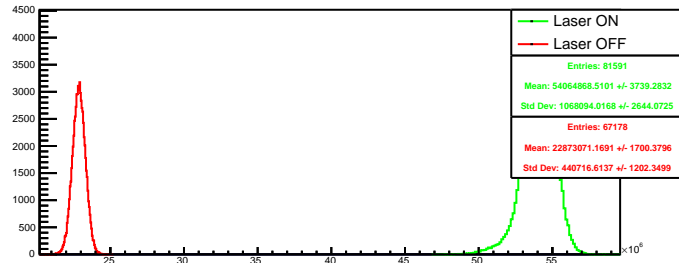
Run 4532 quartetwise, summ4: Beam ON
