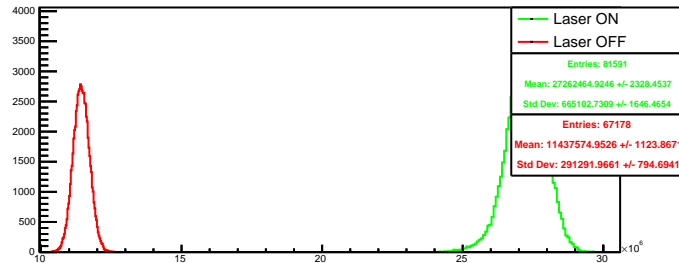
Run 4532 quartetwise, negH4: Beam ON
