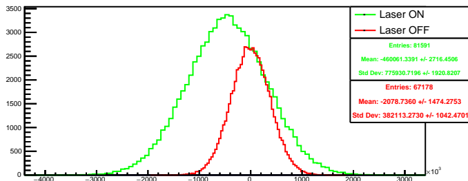
Run 4532 quartetwise, diff4: Beam ON
