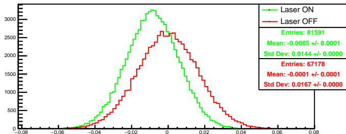
Run 4532 quartetwise, asym4: Beam ON
