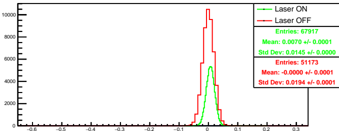
Run 4535 quartetwise, asym0: Beam ON
