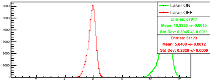
Run 4535 quartetwise, posH0: Beam ON
