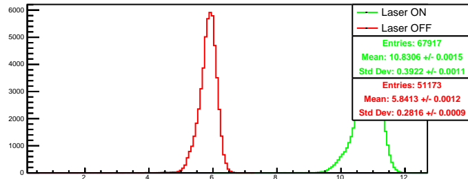
Run 4535 quartetwise, negH0: Beam ON
