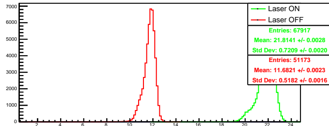
Run 4535 quartetwise, summ0: Beam ON
