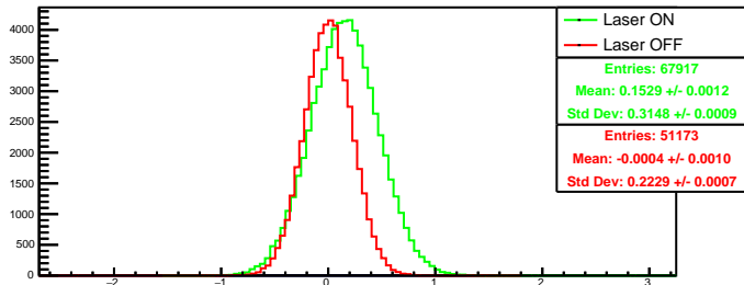
Run 4535 quartetwise, diff0: Beam ON
