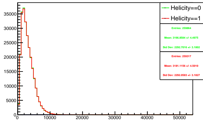
Run 4536 triggerwise, sums: Beam ON, Laser OFF
