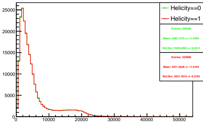
Run 4536 triggerwise, sums: Beam ON, Laser ON
