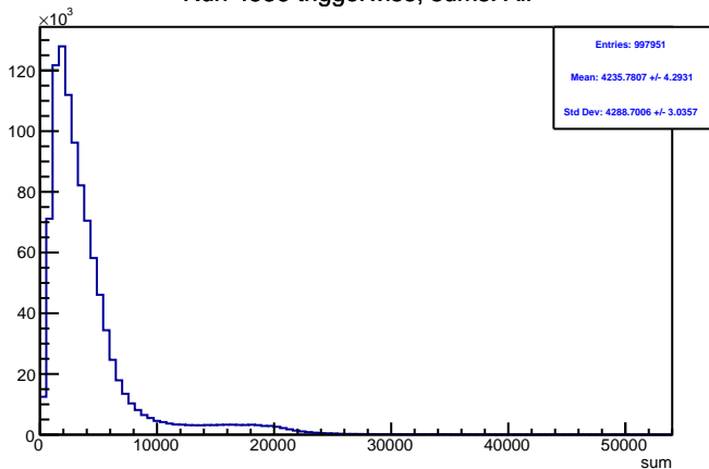
Run 4536 triggerwise, sums: All
