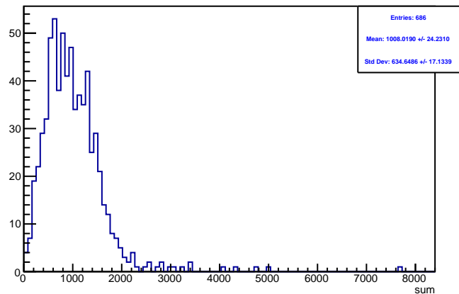
Run 4536 triggerwise, sums: Beam ON, Laser OFF
