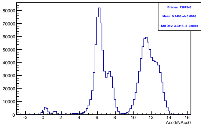
Run 4537 mpwise, acc0: Beam ON, Laser ON
